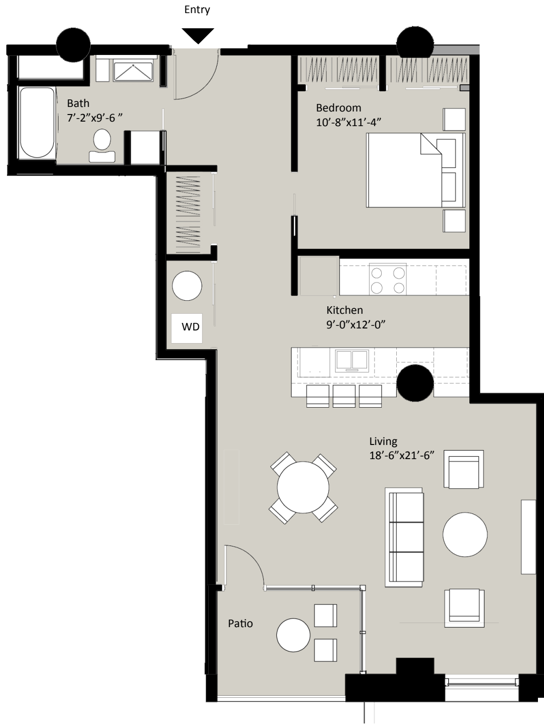
SECOND FLOOR - UNIT 201 ONE BEDROOM UNIT 993 SF + 69 SF PATIO
